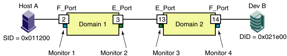
FIGURE 78 Setting end-to-end monitors on a port
